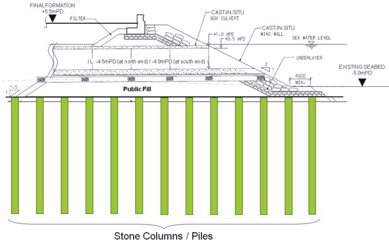
Figure 25 - Seawall Formation in Portion D (Sheet 2 of 3)
